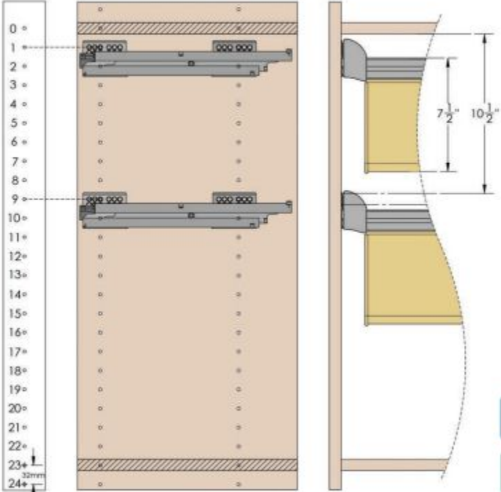
divided deep drawers 31.6385.(WIDTH).(FABRIC).(FINISH)
